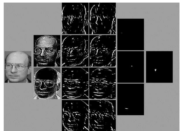
Figure 2. Propagation of activity within the face detection network described by Van Rullen et al [7].
