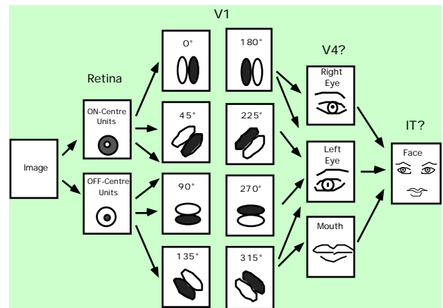
Figure 2. A simple three layer feed-forward architecture that is capable of accurate face identification [7].
